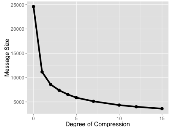
Figure 8: System-wide communication volume resulting from the use of different lossy compression degrees.
