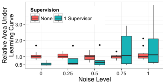
Figure 10: Robustness of experience sharing to the use of sub-optimal/corrupted context features.
