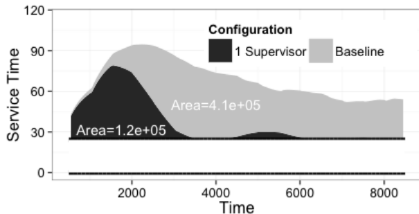
Figure 4: Performance of the single-supervisor configuration vs. no-sharing. Smaller areas under the curve indicate faster convergence.
