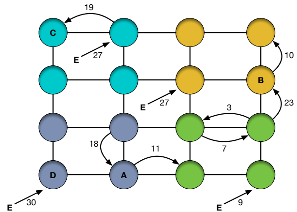
Figure 1: Sample task allocation network.
