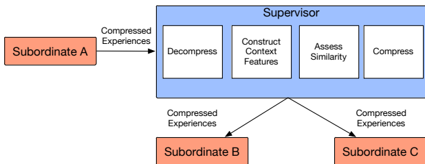
Figure 7: Relaying compressed experiences through a supervisor.
