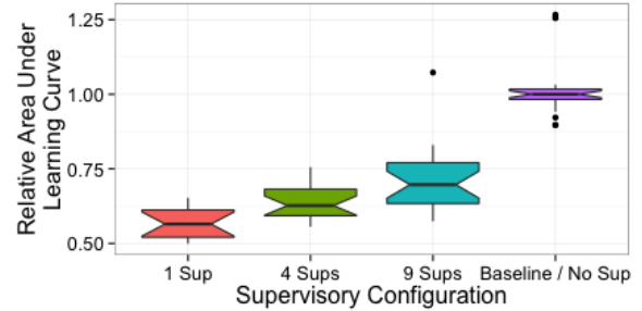
Figure 5: Performance of different supervisory configurations in a 100-agent network; smaller values correspond to faster learning.
