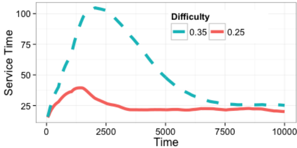
Figure 3: Performance under different difficulty settings \lambda .
