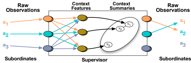
Figure 2: Overview of the context-based transfer process.
