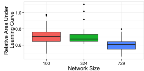
Figure 6: Performance of the 9-supervisor configuration as a function of network size.
