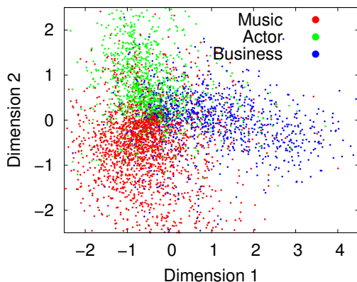
Figure 3: 2-d vector distribution of users in the three most common occupations under Tuv. Here we set \Delta t = 1 year.
