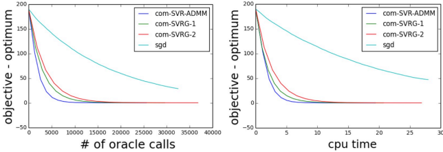
Figure 3: On-policy learning experiment with S = 200, d = 100 .
