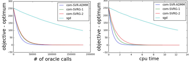
Figure 2: Portfolio Management with cov = 10 . The other parameters have the same value as Figure 1.
