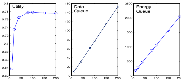
Fig. 3. Average utility, average data queue size and average energy queue size under OSA.
