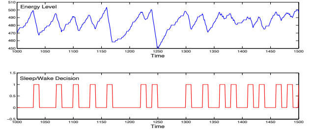
Fig. 5. A sample path energy level process and a sample path sleep/wake decision process under V = 40 from time 1000 to 1500.
