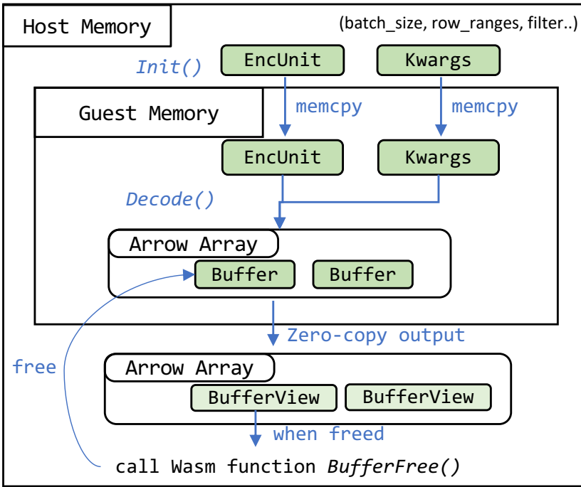
Fig. 8. Wasm Decoding Implementation – An overview of F3’s decoding procedure for an EncUnit using Wasm. Buffers residing in guest memory will be freed once the reference count of the BufferView in the host gets to zero. We omit the call to Check() for brevity.
