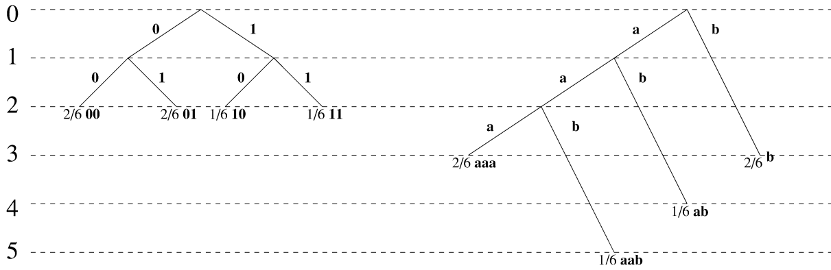
Fig. 2. Two min-cost prefix-free codes for probabilities 2/6, 2/6, 1/6, 1/6 , and their tree representations. The code on the left is optimal for c_1 = c_2 = 1 while the code on the right, the prefix-free code from Fig. 1, is optimal for c_1 = 1, c_2 = 3 .
